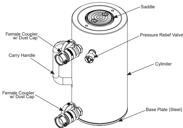
Figure 1 - Typical HUD Series Cylinder Components
